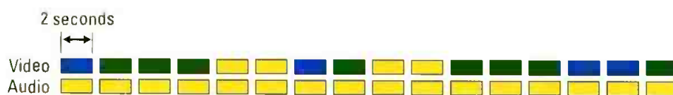
Figure 1. Adaptive streaming requires the video be cut into small segments and then encoded into various bit rates prior to transmission.
