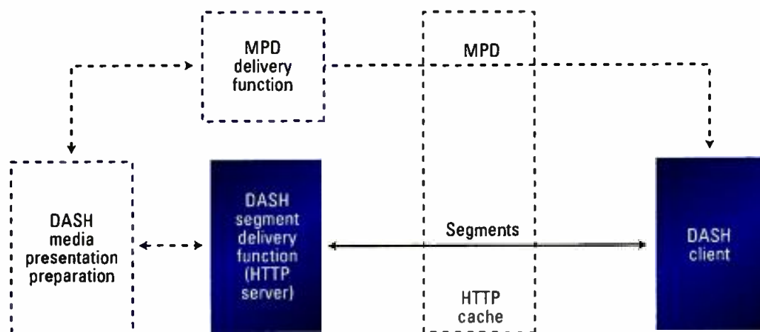
Figure 1. MPEG-DASH defines a standard set of Media Presentation Description and Segment Formats that enable adaptive bit rate IP video streaming.
